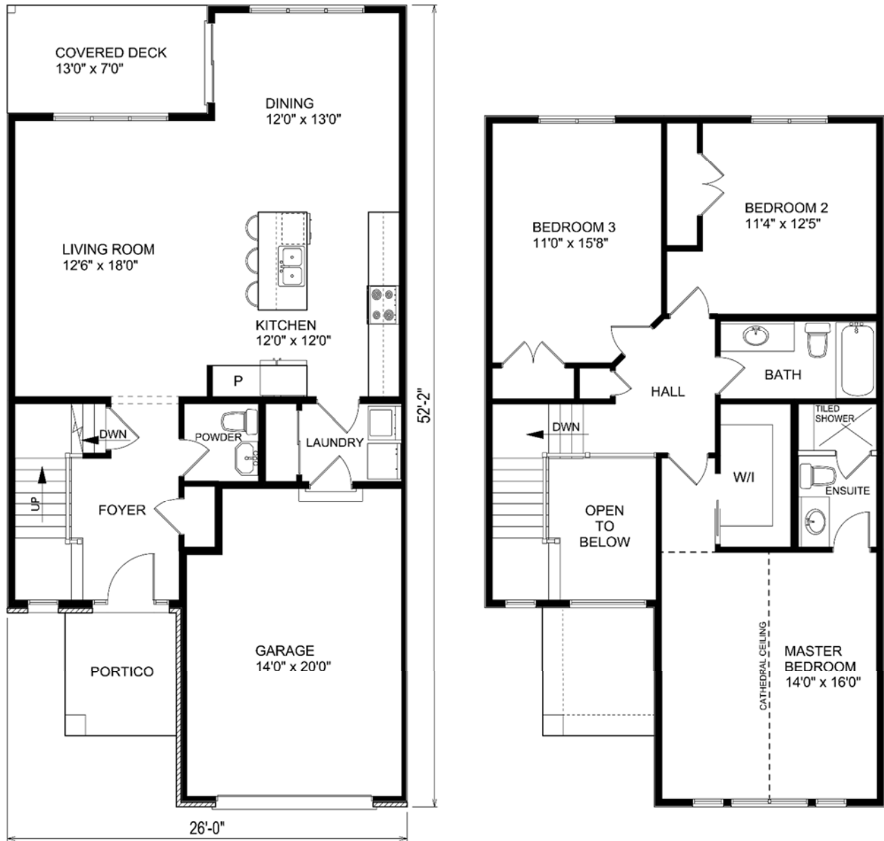
FLOOR PLAN
