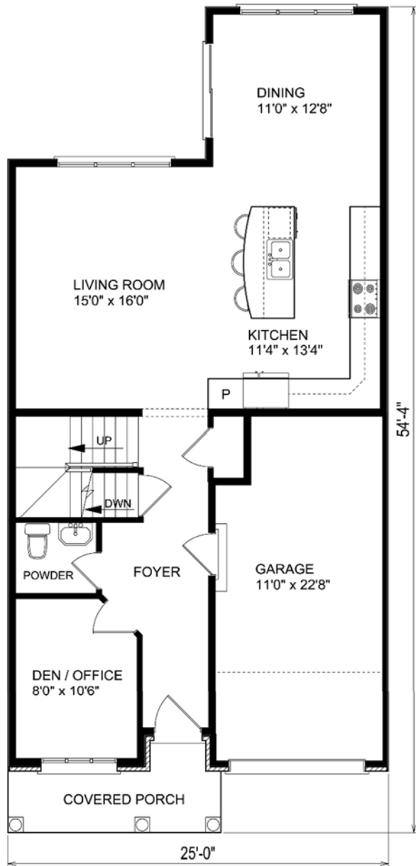
FLOOR PLAN
