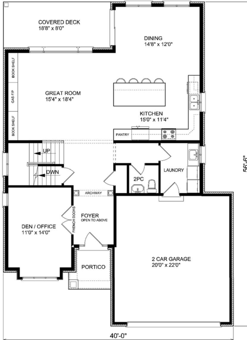
FLOOR PLAN
