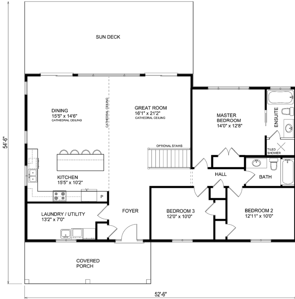
FLOOR PLAN
